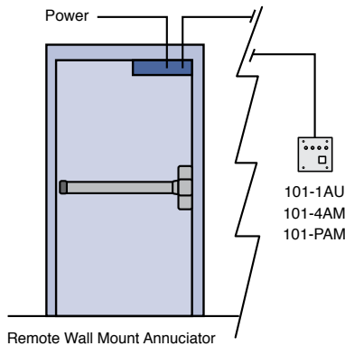
Remote Wall Mount Annunciator
