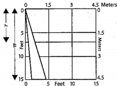
Side view of coverage range with -14° aim
